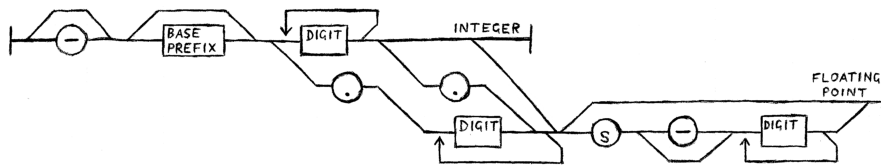
Figure 3.1: Syntax diagram for numerical input
